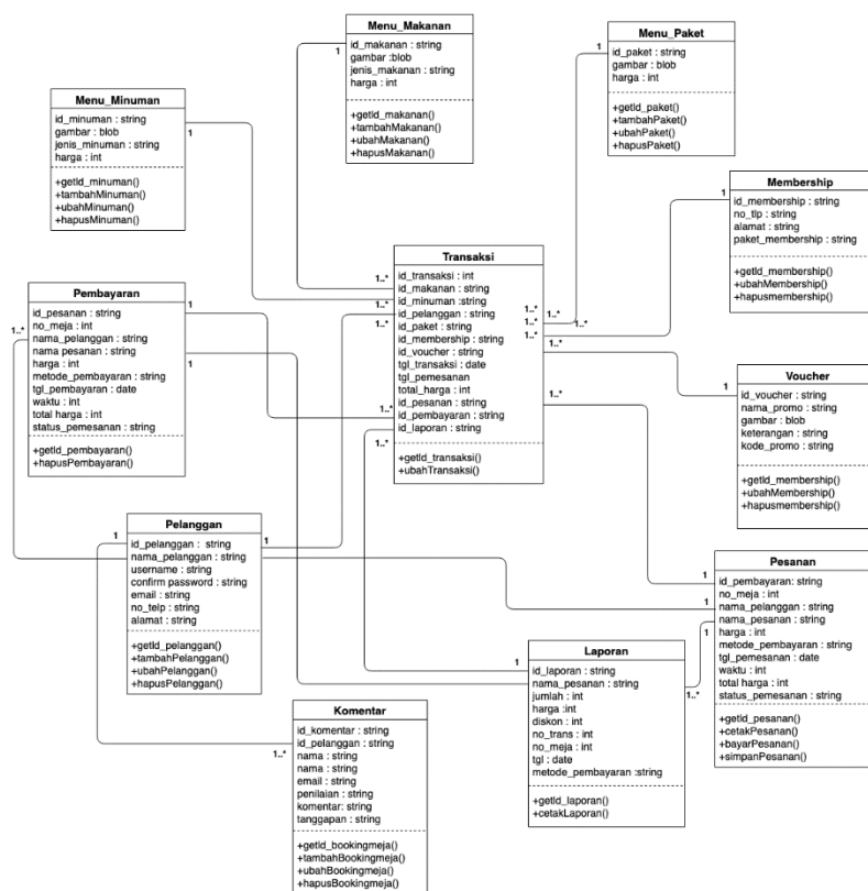
Gambar 5. Class Diagram
